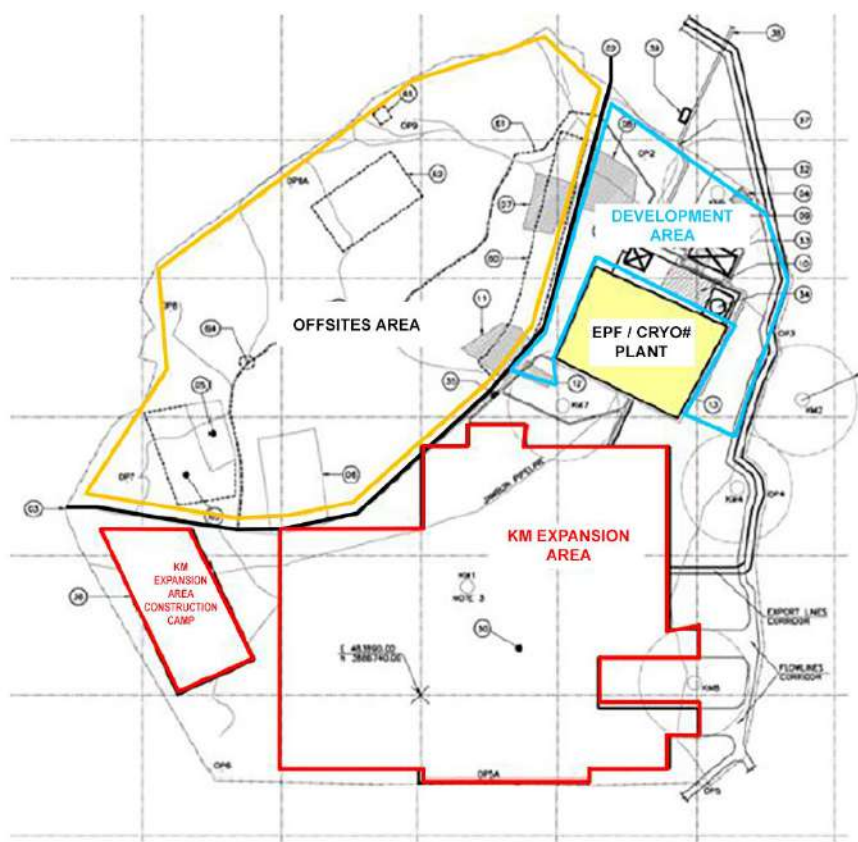
Figure 2-3 KM site plan
